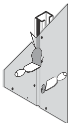
3. Fill the joint 100% and apply a thin layer of the mix on the joint (2.7" width)
