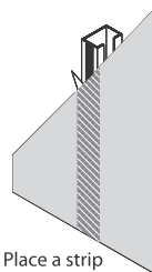
4. Place a strip of joint mesh along the joint. Secure it on the surface with a trowel
